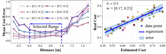
Figure 9: Left: The difference between the estimated cost by (26) and the measured cost under different weights w , for different choice of the distance d(q_n, q_{n+1}) . Right: The difference actual with 40 samples, when w = [0.17, 0.23]^T and d = 0.5 .
