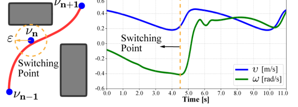
Figure 8: Illustration of the smooth transition strategy in (25) when the agent switches from one intermediate waypoint to another. The switch function \eta_\epsilon is activated once the current waypoint is reached with a margin \epsilon . The resulting trajectory and control inputs are all smooth.
